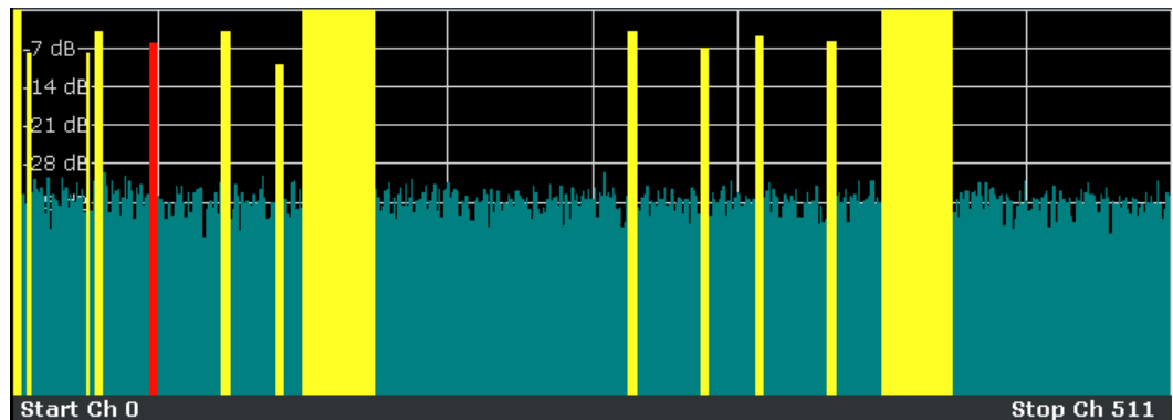
Fig. 6-1: Code Domain Power Display for R&S FSV-K72
